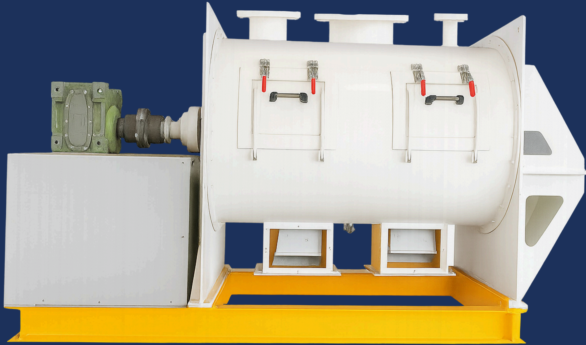
2000 Ltr Plough Shear Mixer.
