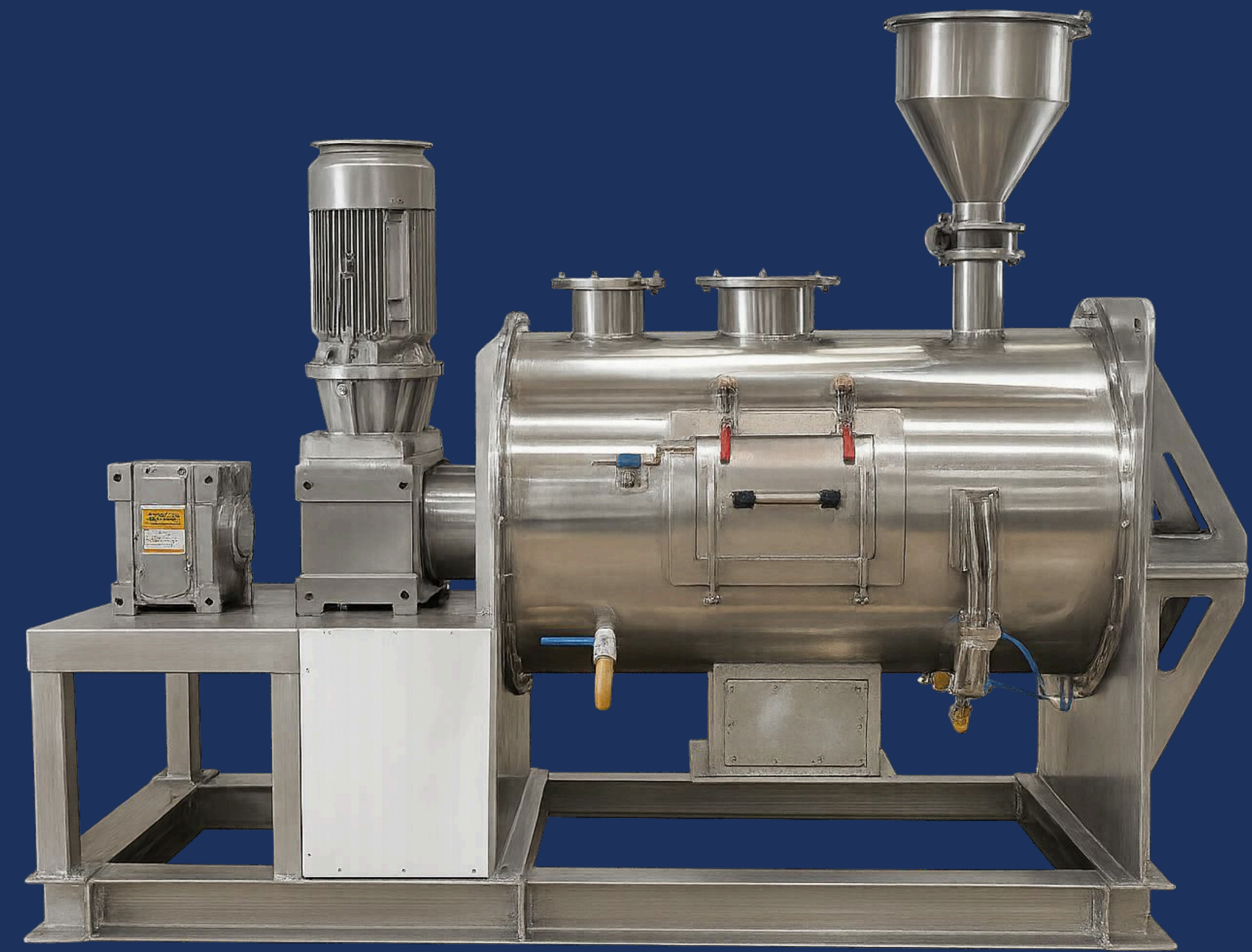
300 Ltr Plough Shear Mixer.
